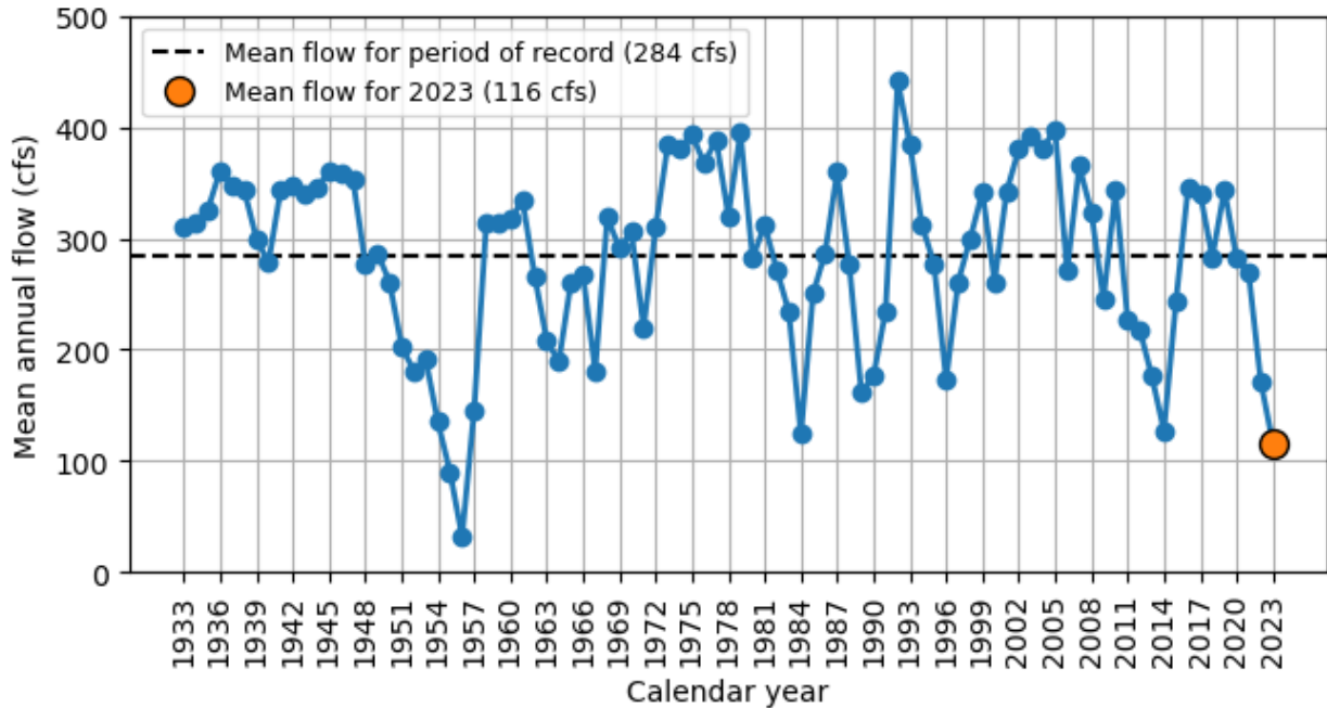
Figure 3. Historical time series of mean annual flow at Comal Springs.
