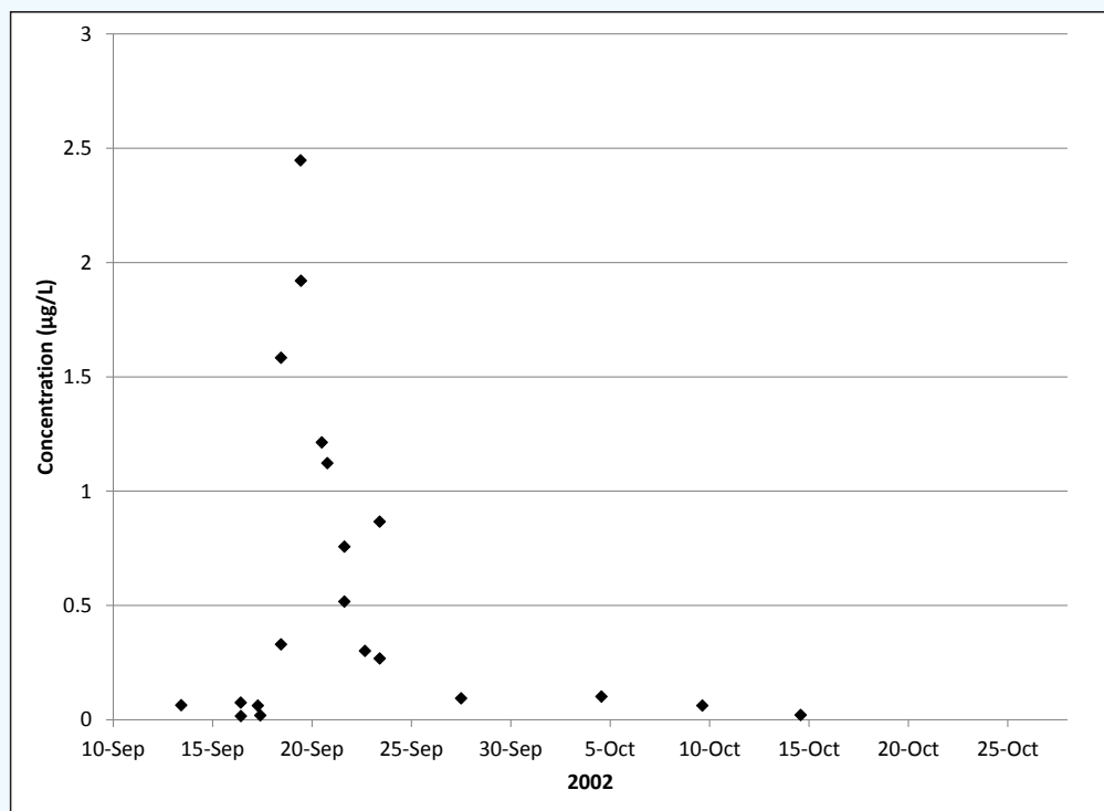
Figure 15. Breakthrough Curve for Wonder World Cave for September 16, 2002 Tracer Test
