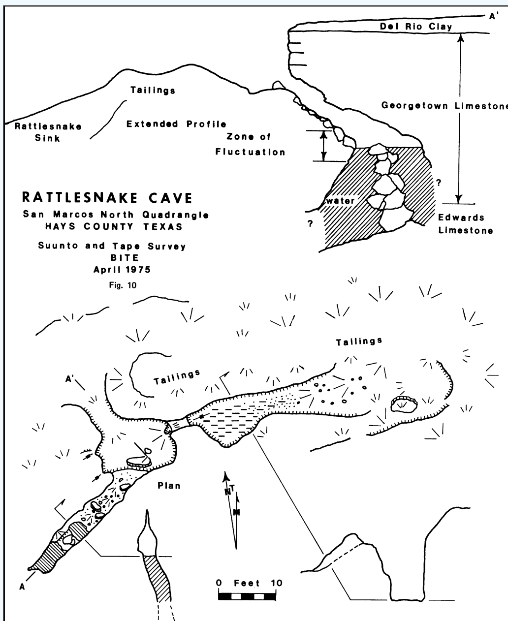
Figure 44. Map of Rattlesnake Cave
