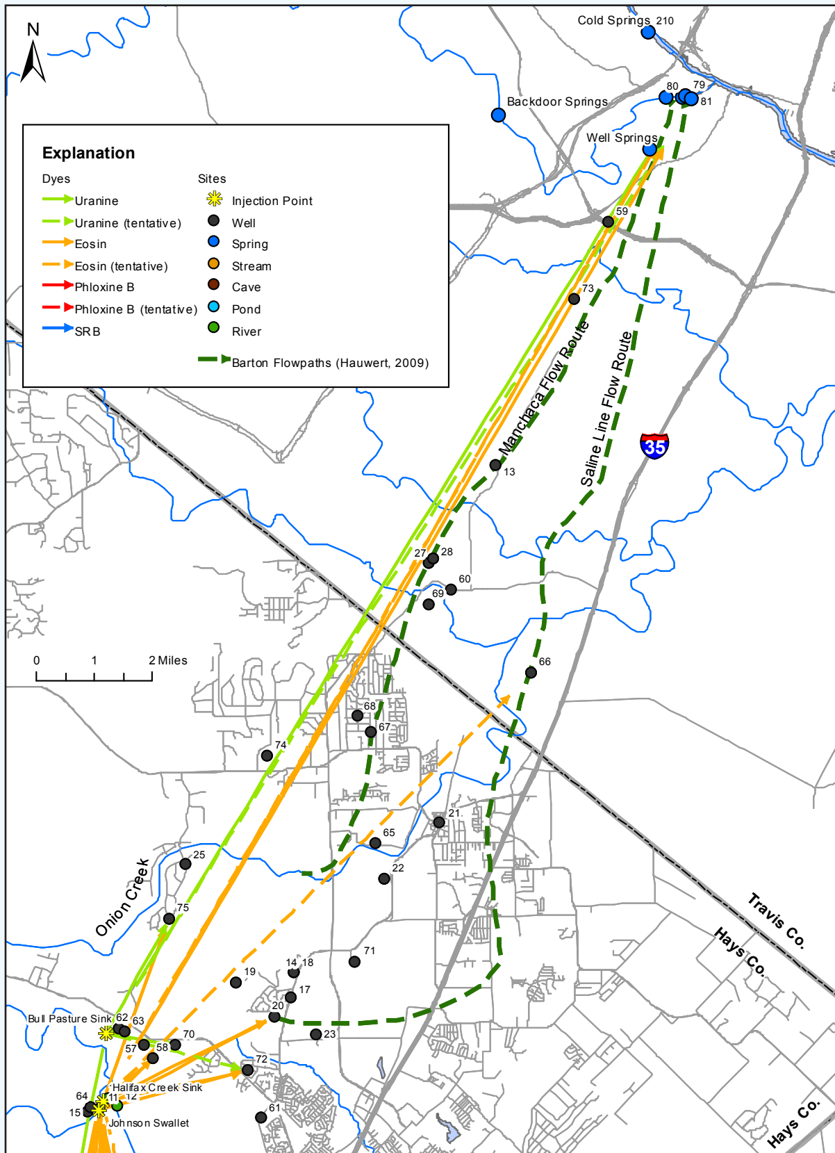
Figure 32. Tracer-Test Results North of the Blanco River
