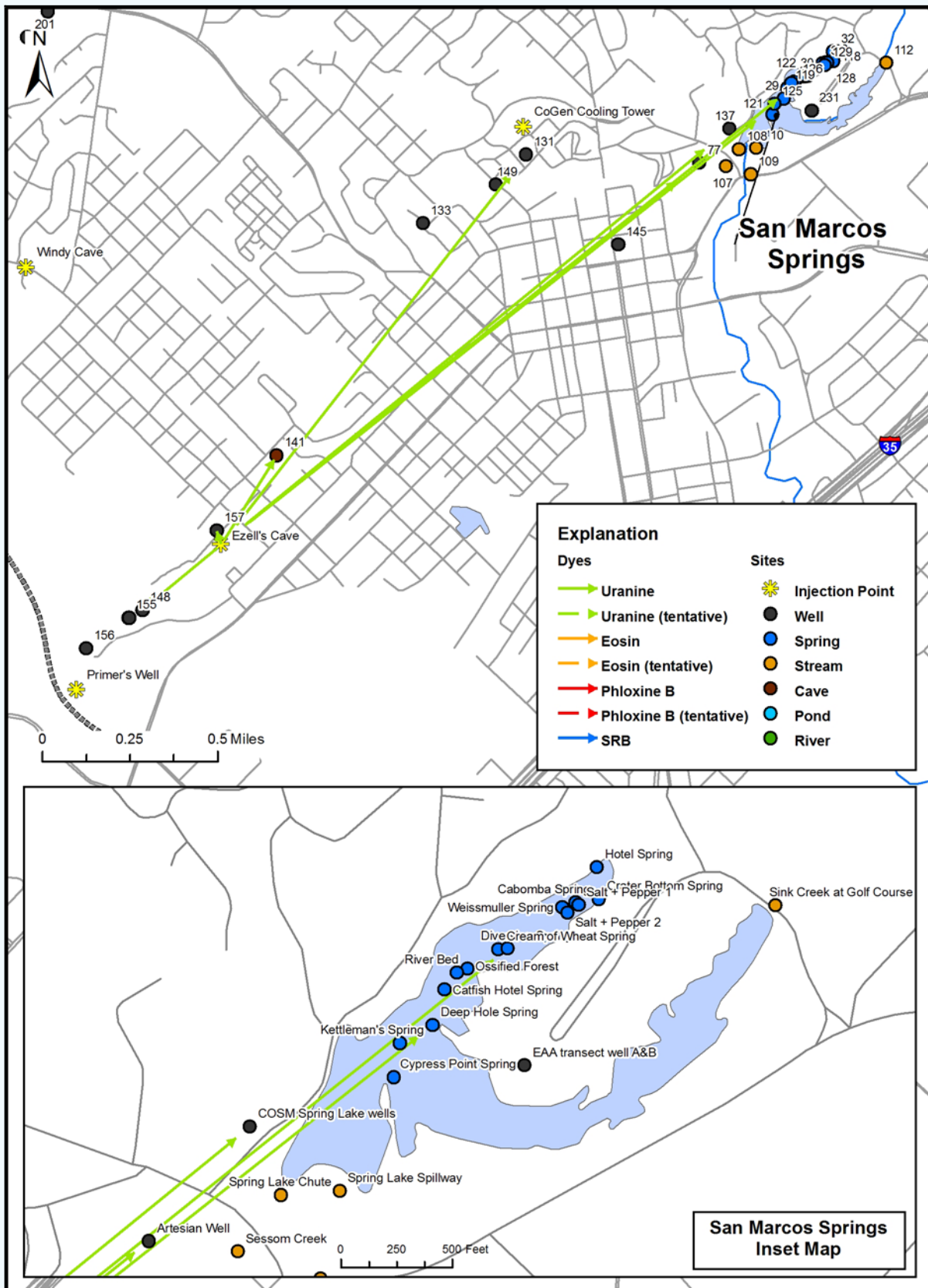
Figure 14. Southwestern Tracer Tests—September 16, 2002, Results
