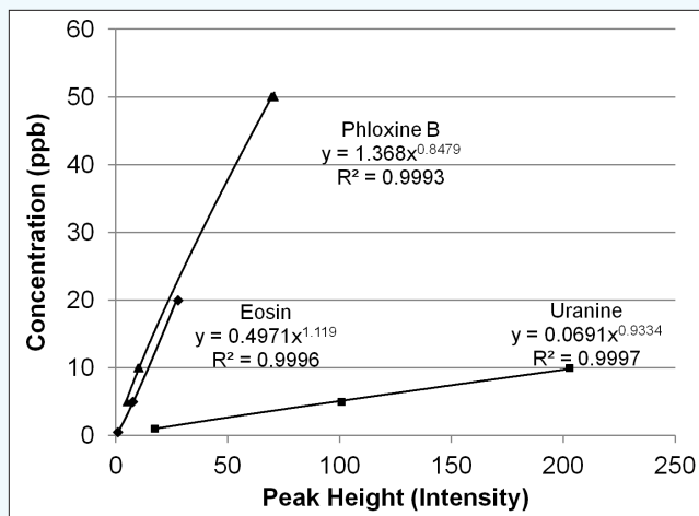
Figure 7. Example of Regression Curves for Dye Standards
