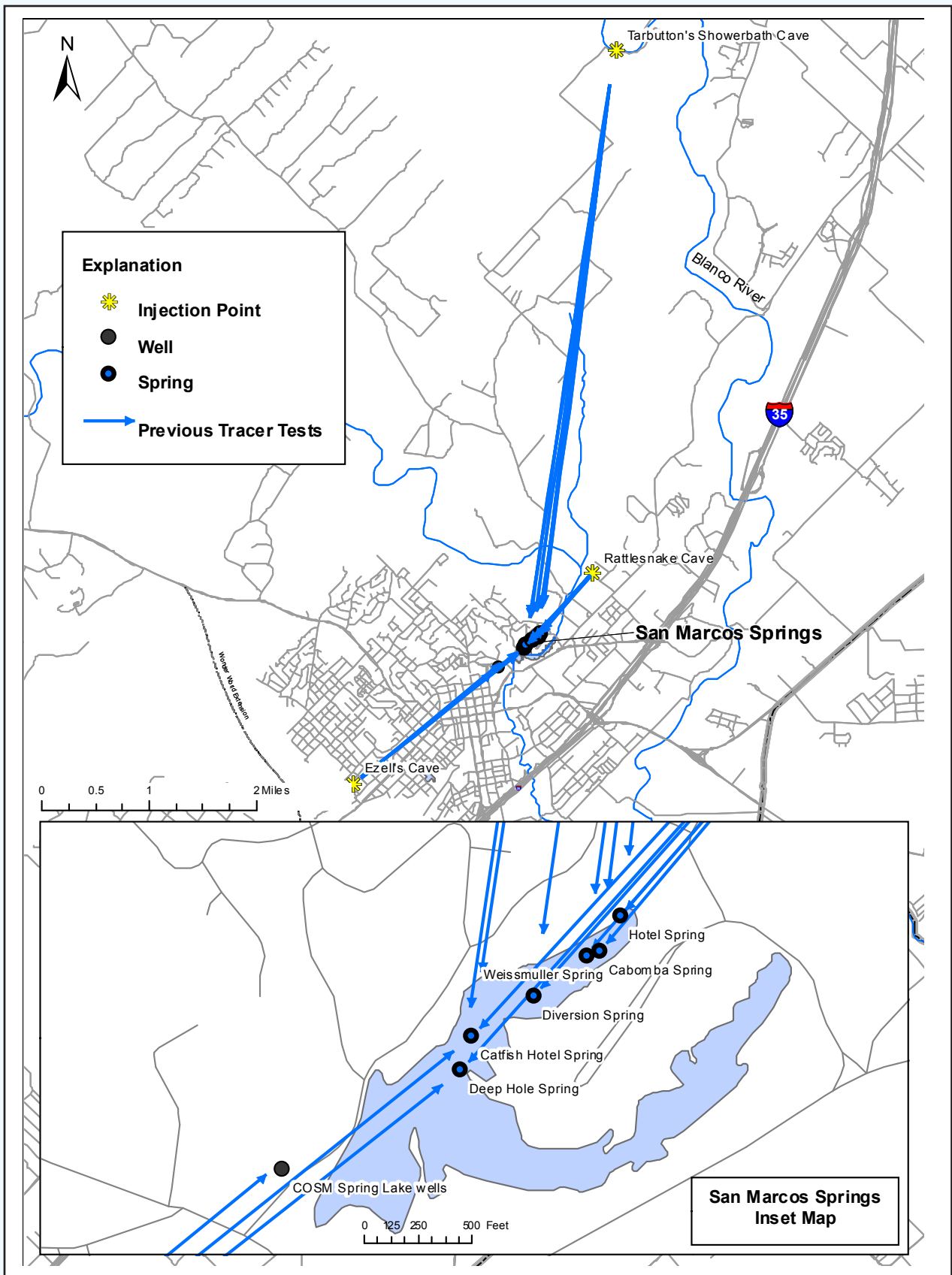
Figure 5. Previous Tracer Tests at San Marcos Springs
