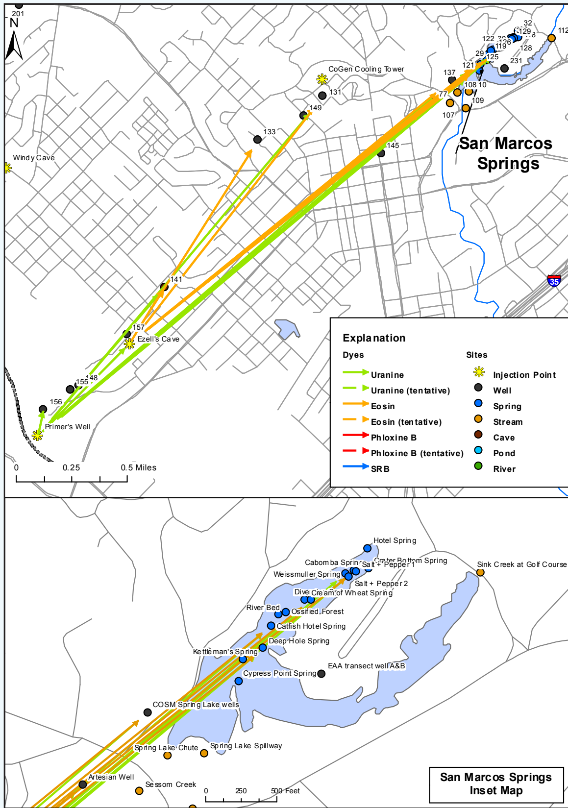
Figure 17. Southwestern Tracer Tests—January 2004
