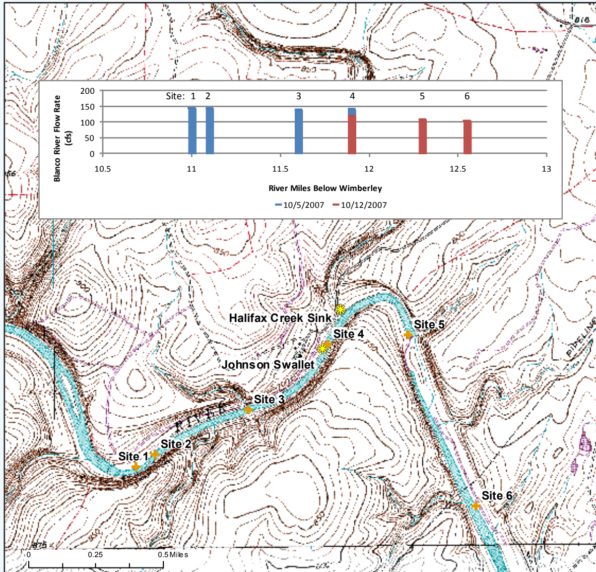
Figure 27. Flow Survey of the Blanco River along Halifax Ranch, October 2007. Flow Measured by Marcus Gary, Nico Hauwert (COA), and Joseph Beery (BSEACD)
