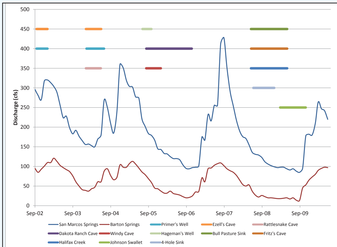
Figure 9. Tracer-Test Durations Compared with Discharge at San Marcos and Barton Springs
