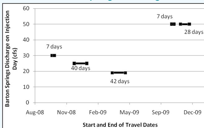
Figure 51. Evaluation of Travel Time and Barton Springs Discharge
