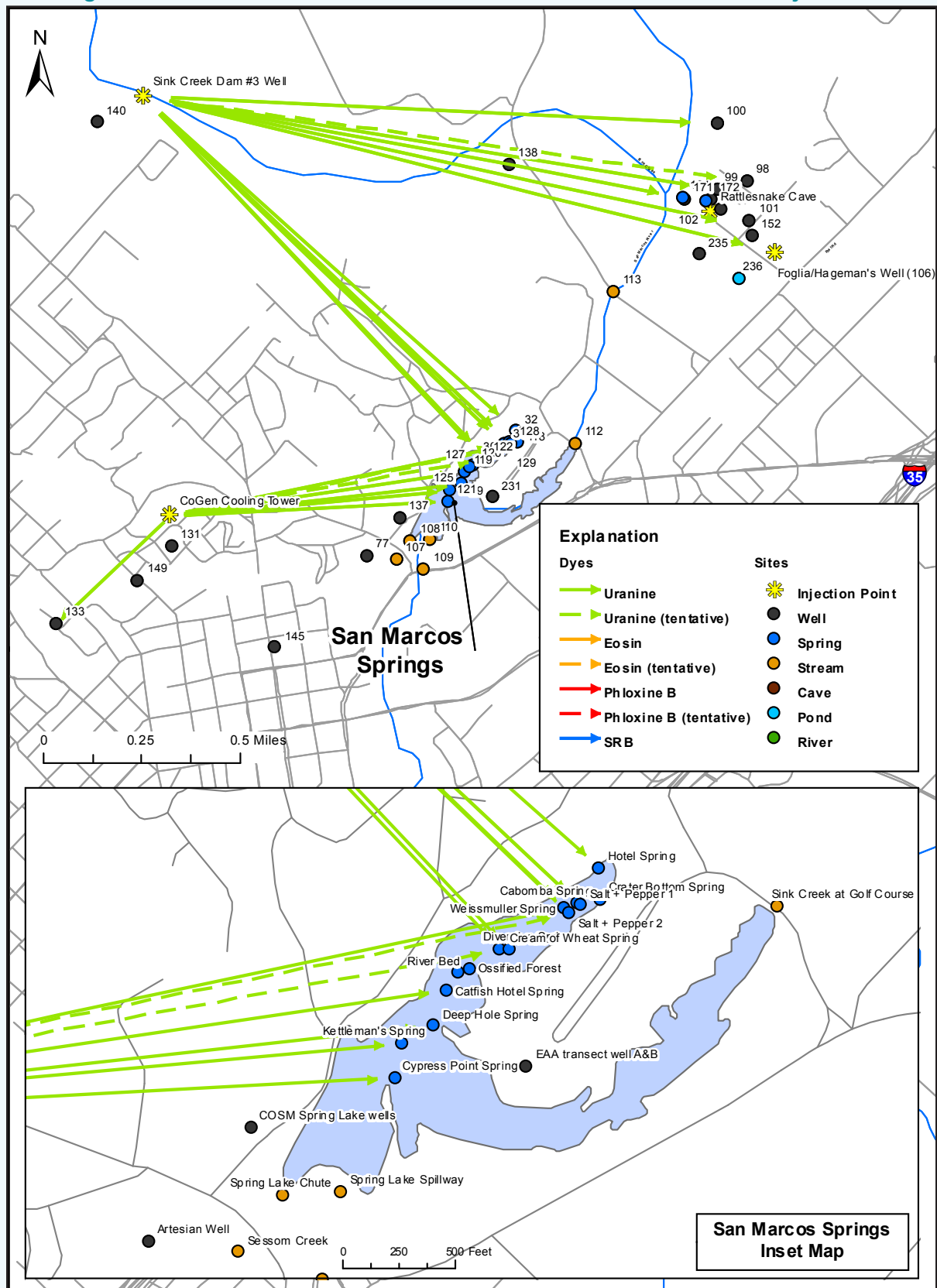
Figure 43. Northern Tracer-Test Results from Sink Creek Dam #3 Injections
