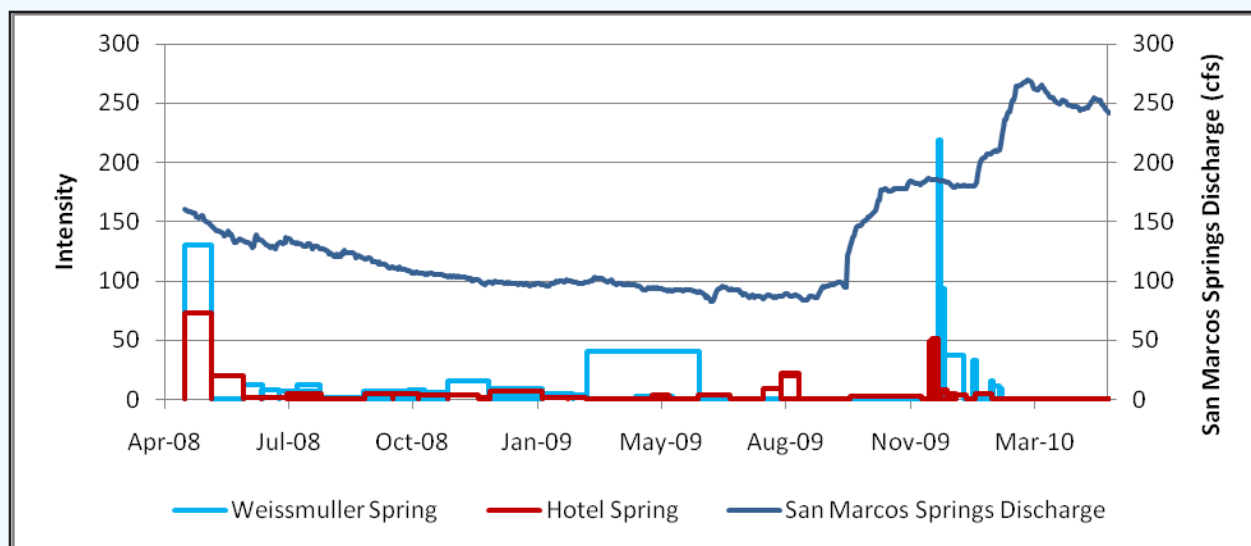
Figure 46. Phloxine B Concentrations in Charcoal Receptors at Hotel and Weissmuller Springs after 2009 Rattlesnake Cave Injection
