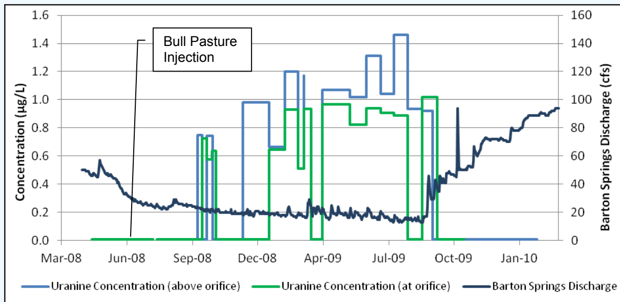
Figure 36. Breakthrough Curves for Uranine in Barton Springs
