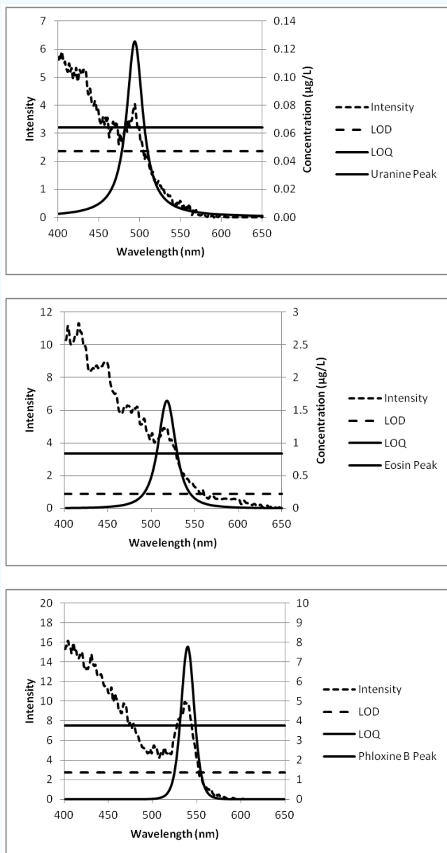
Figure 8. Calculation of LOD and LOQ for Uranine, Eosin, and Phloxine B
