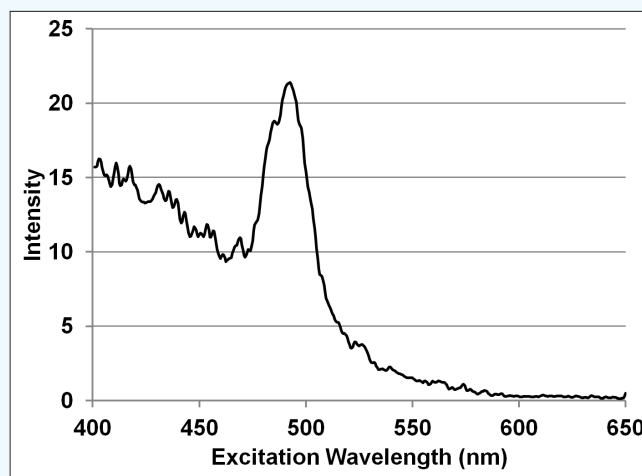
Figure 6. Typical Spectrograph of Uranine Dye from the LS-50B
