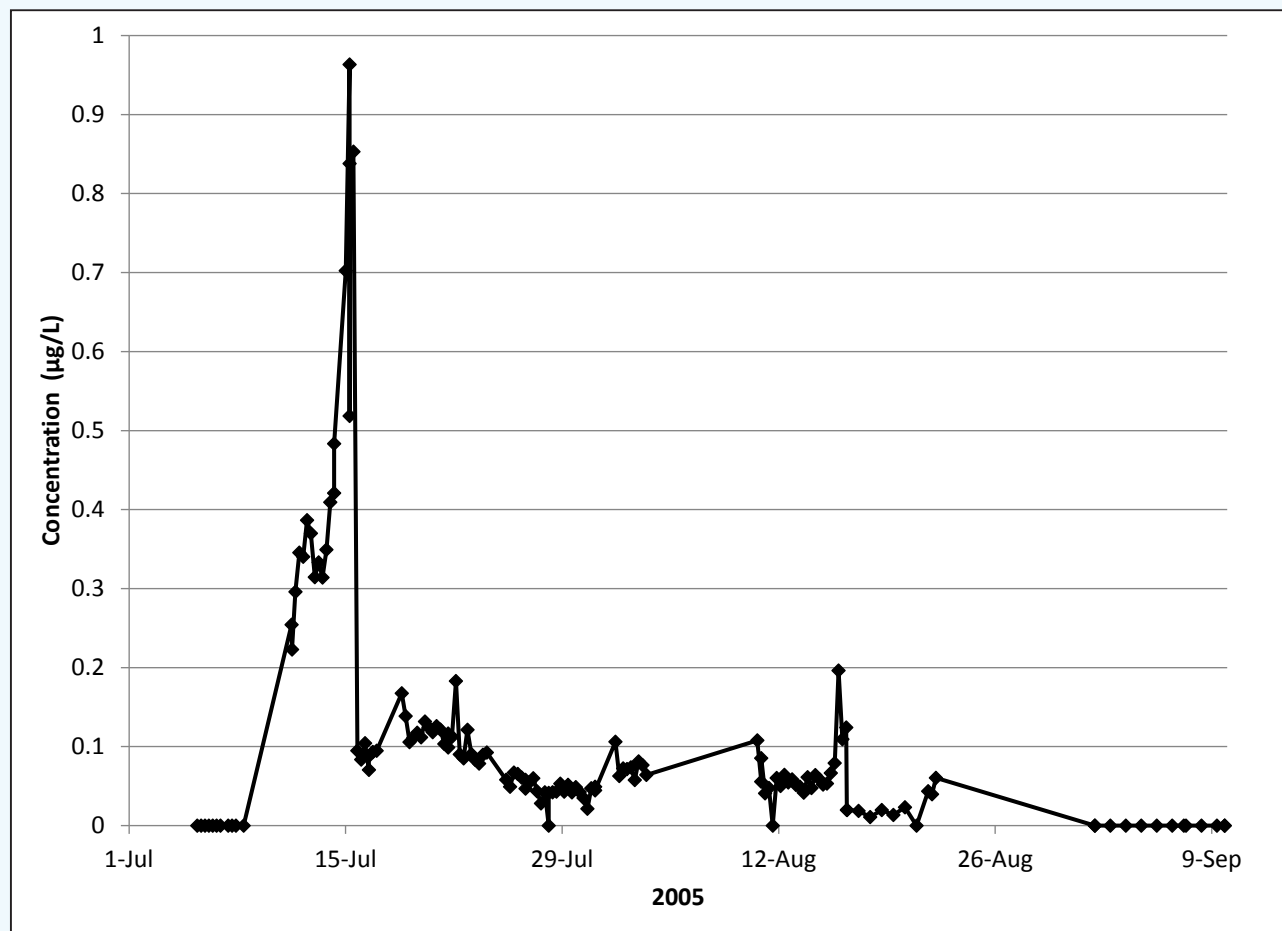
Figure 22. Breakthrough Curve for Deep Hole Spring for July 5, 2005, Tracer Test
