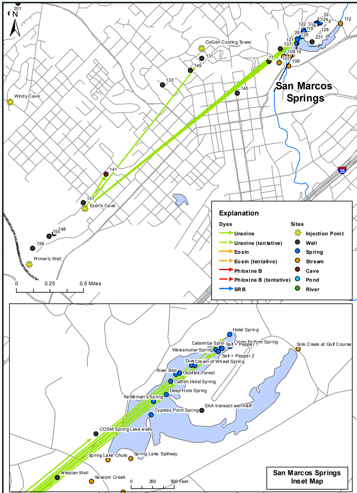
Figure 20. Southwestern Tracer Tests—July 2004 and July 2005
