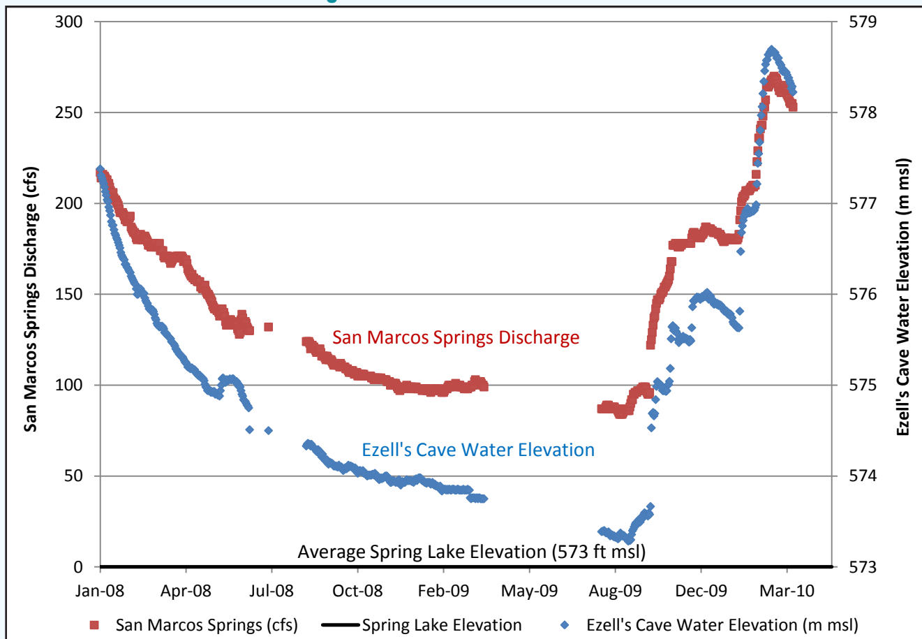
Figure 12. Comparison of San Marcos Springs Discharge with Water Levels in Ezell's Cave
