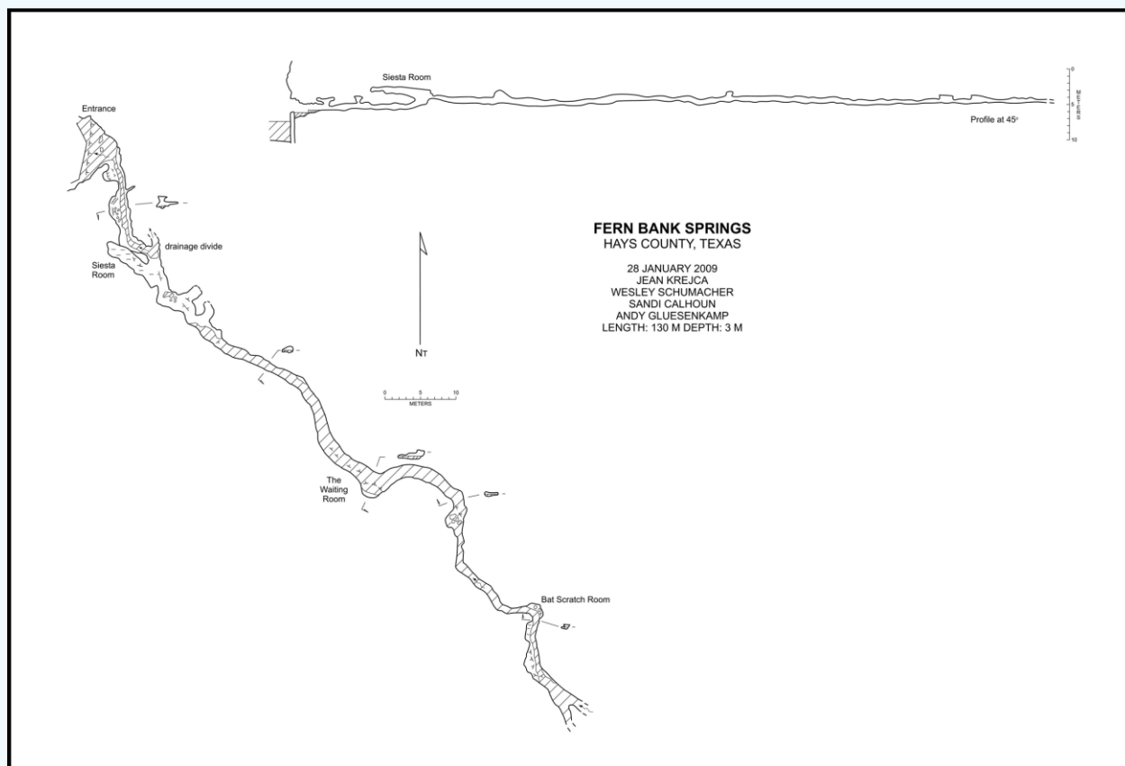
Figure 48. Cave Map of Fern Bank Spring
