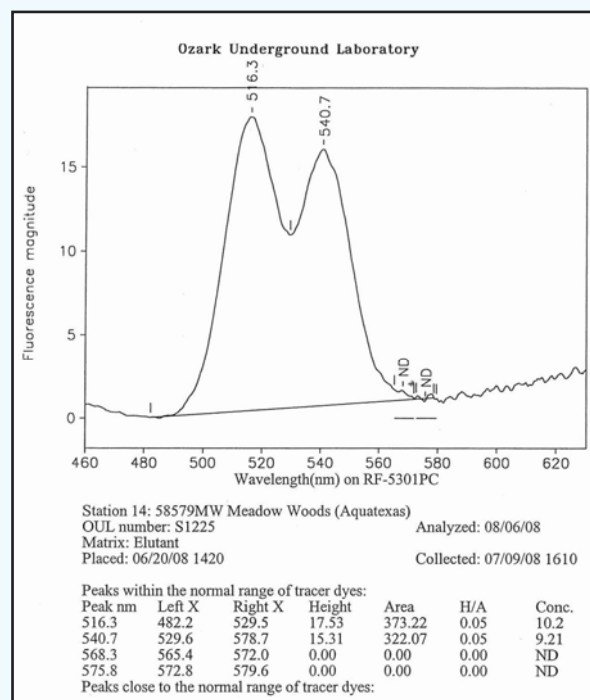
Figure 35. Fluorescence Results from a Charcoal Sample from Meadow Woods Well with Uranine and Eosin Peaks
