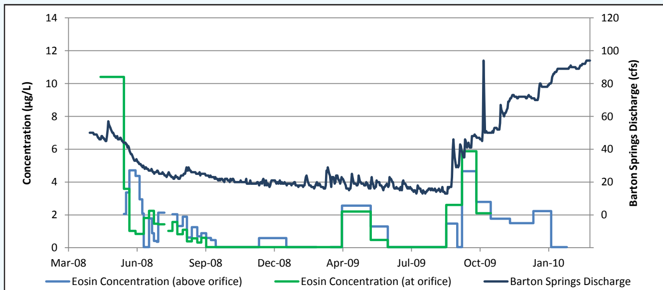
Figure 39. Breakthrough Curves for Eosin at Main Barton Springs in Charcoal Receptors
