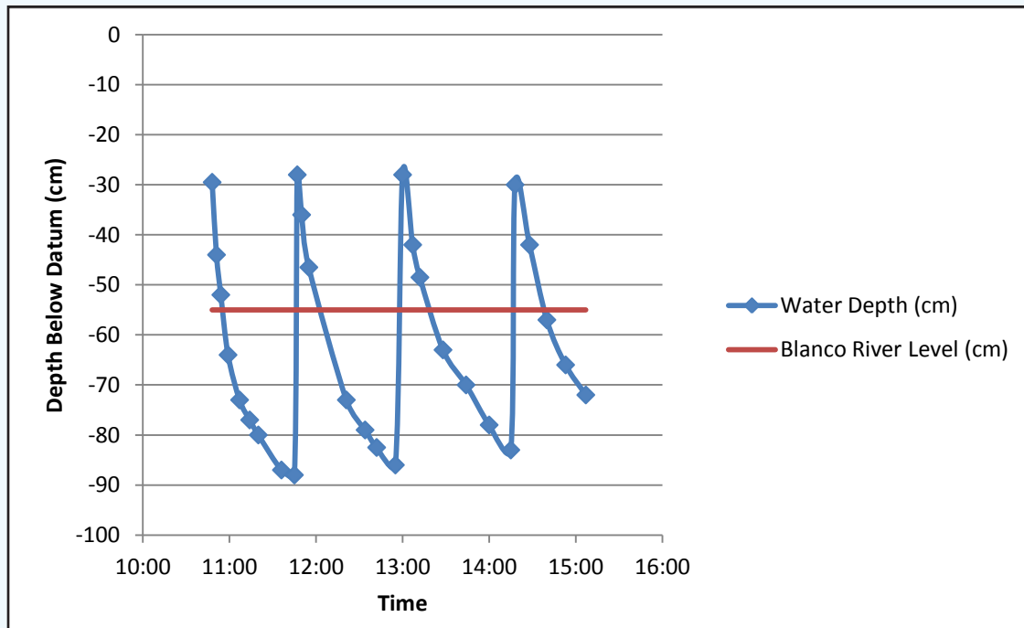
Figure 28. Percolation Test of the Pit Dug in the Approximate Location of the Halifax Sinkhole. Data and Chart from Marcus Gary.
