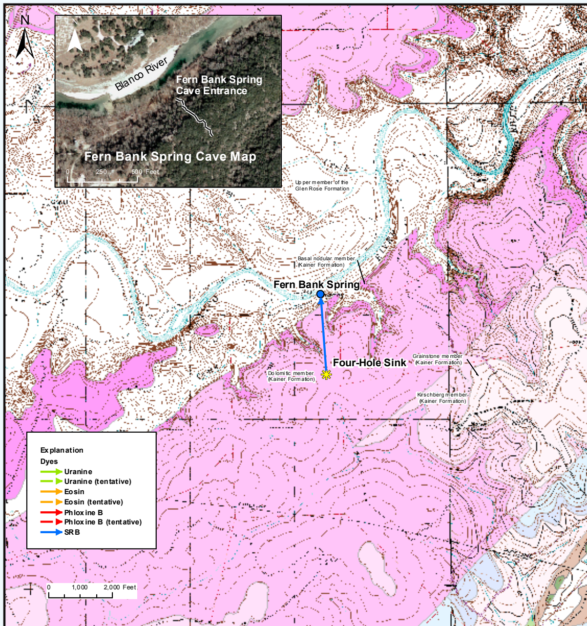
Figure 47. Fern Bank Spring Tracer Test
