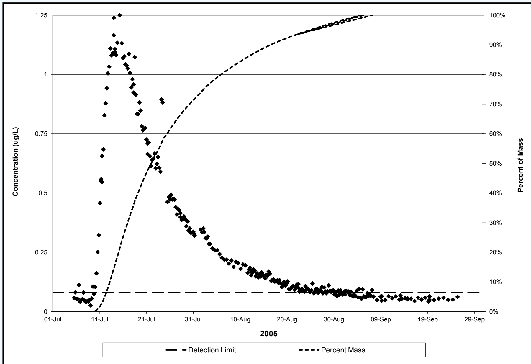
Figure 21. Breakthrough Curve for Artesian Well Showing Percent of Dye Mass for July 5, 2005, Tracer Test
