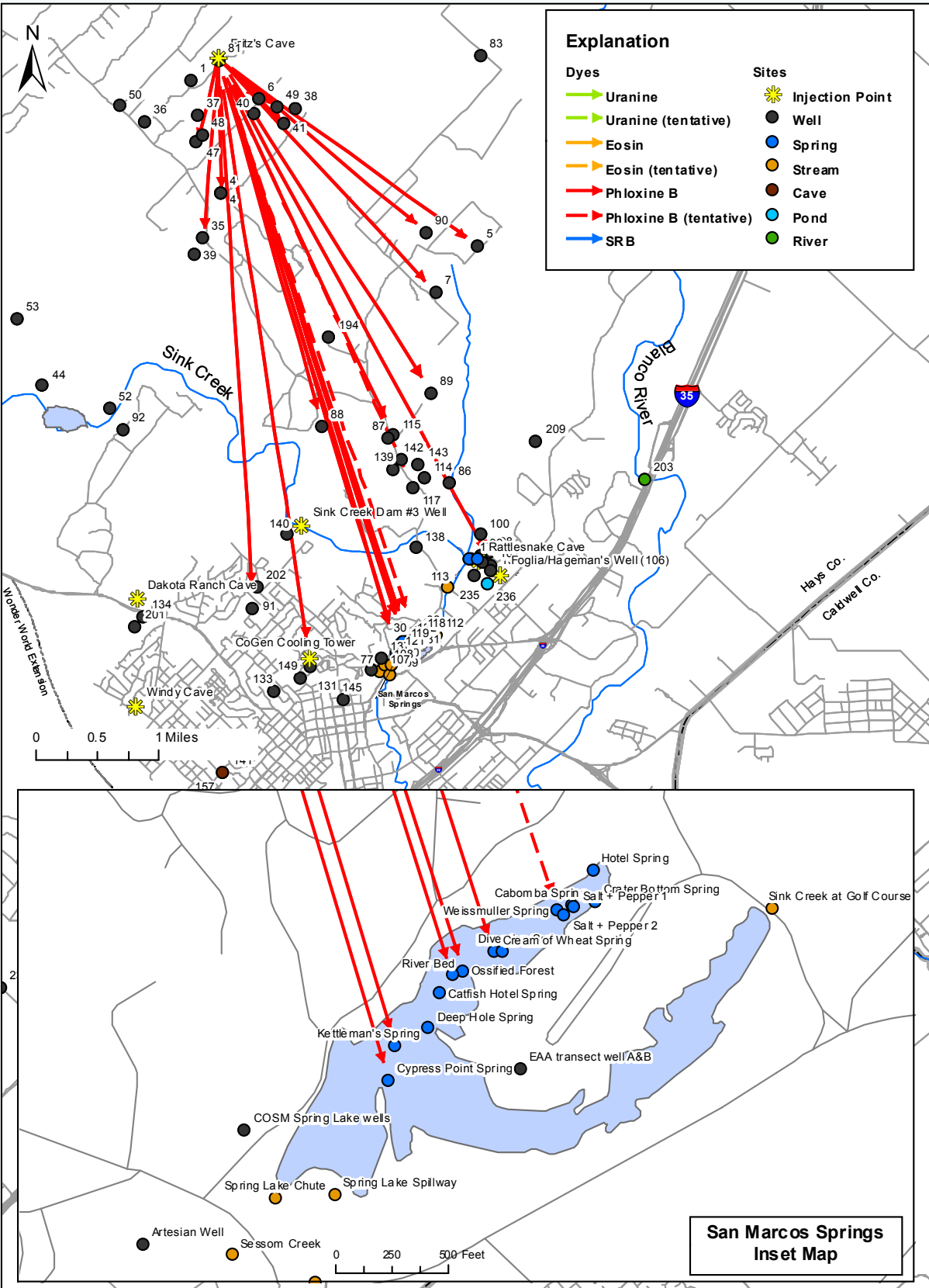
Figure 42. Northern Tracer-Test Results from Fritz's Cave Injections
