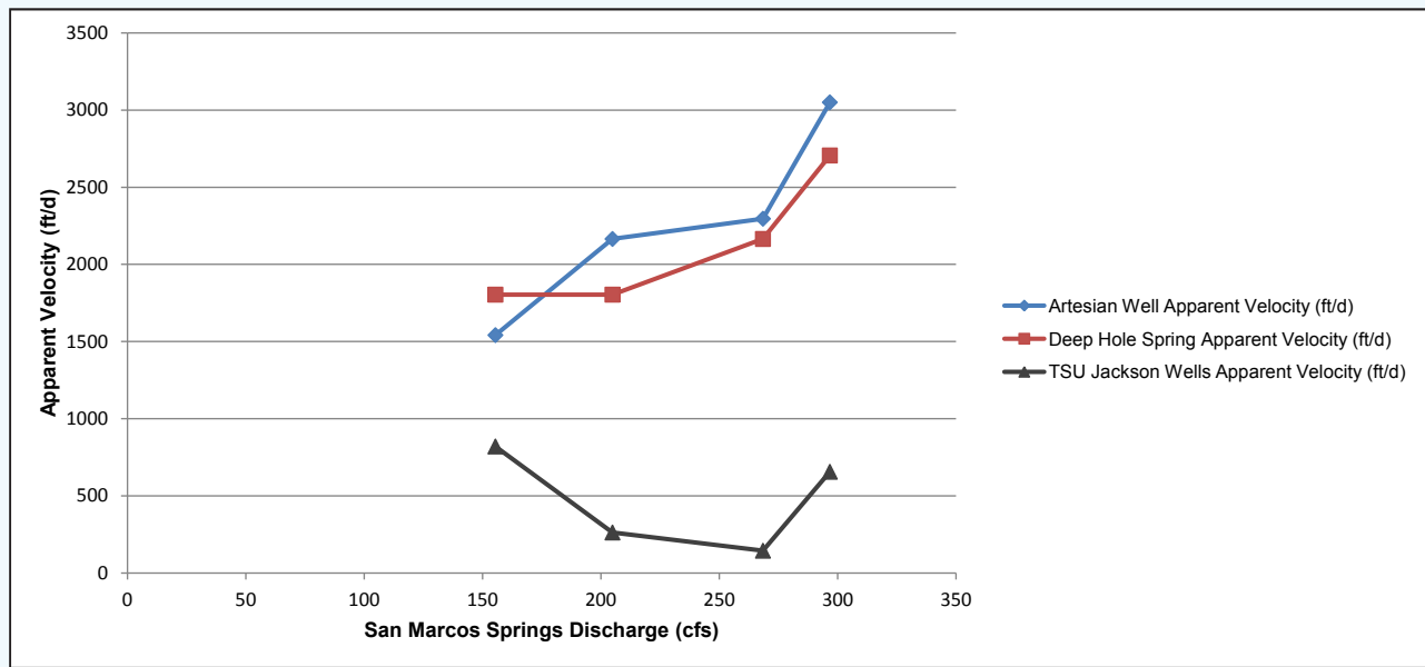
Figure 23. Comparison of Apparent Velocities from Southwestern Tracer Tests
