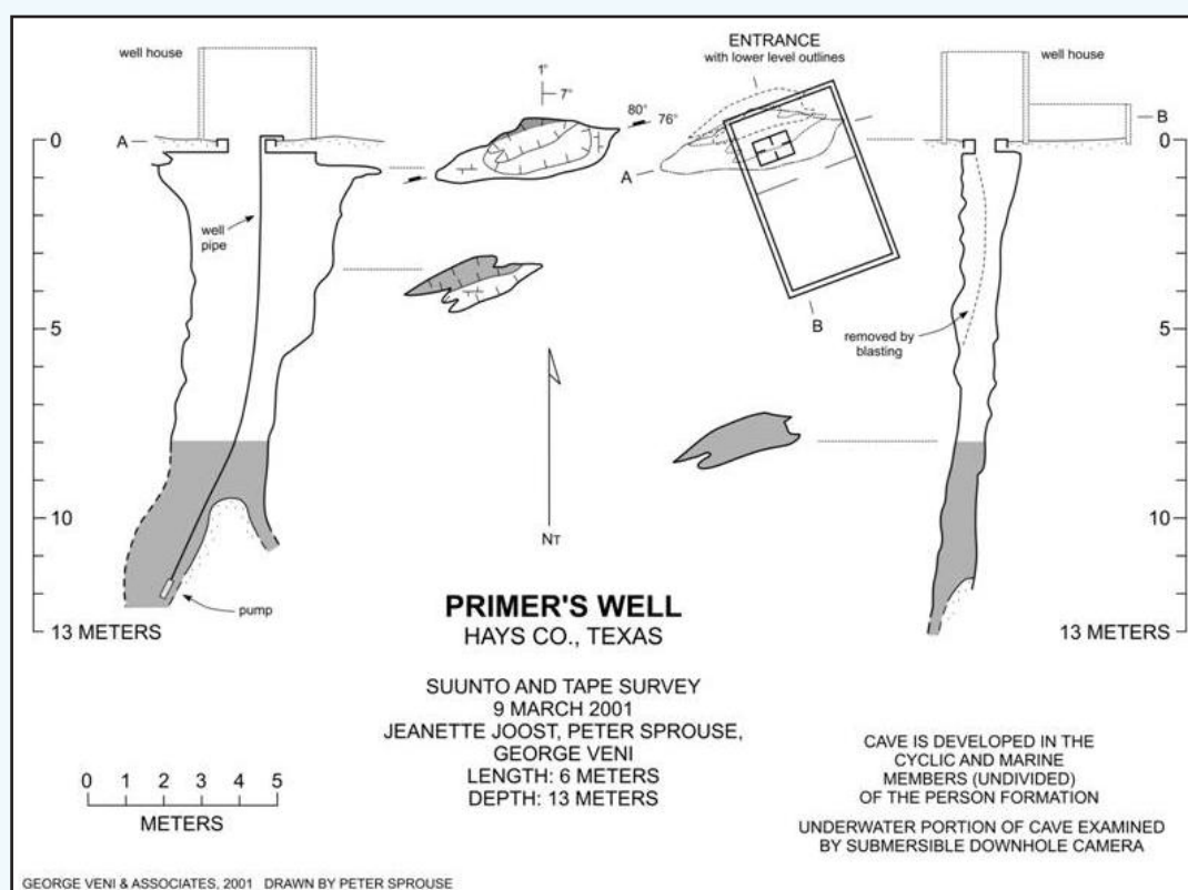
Figure 10. Map of Primer's Well
