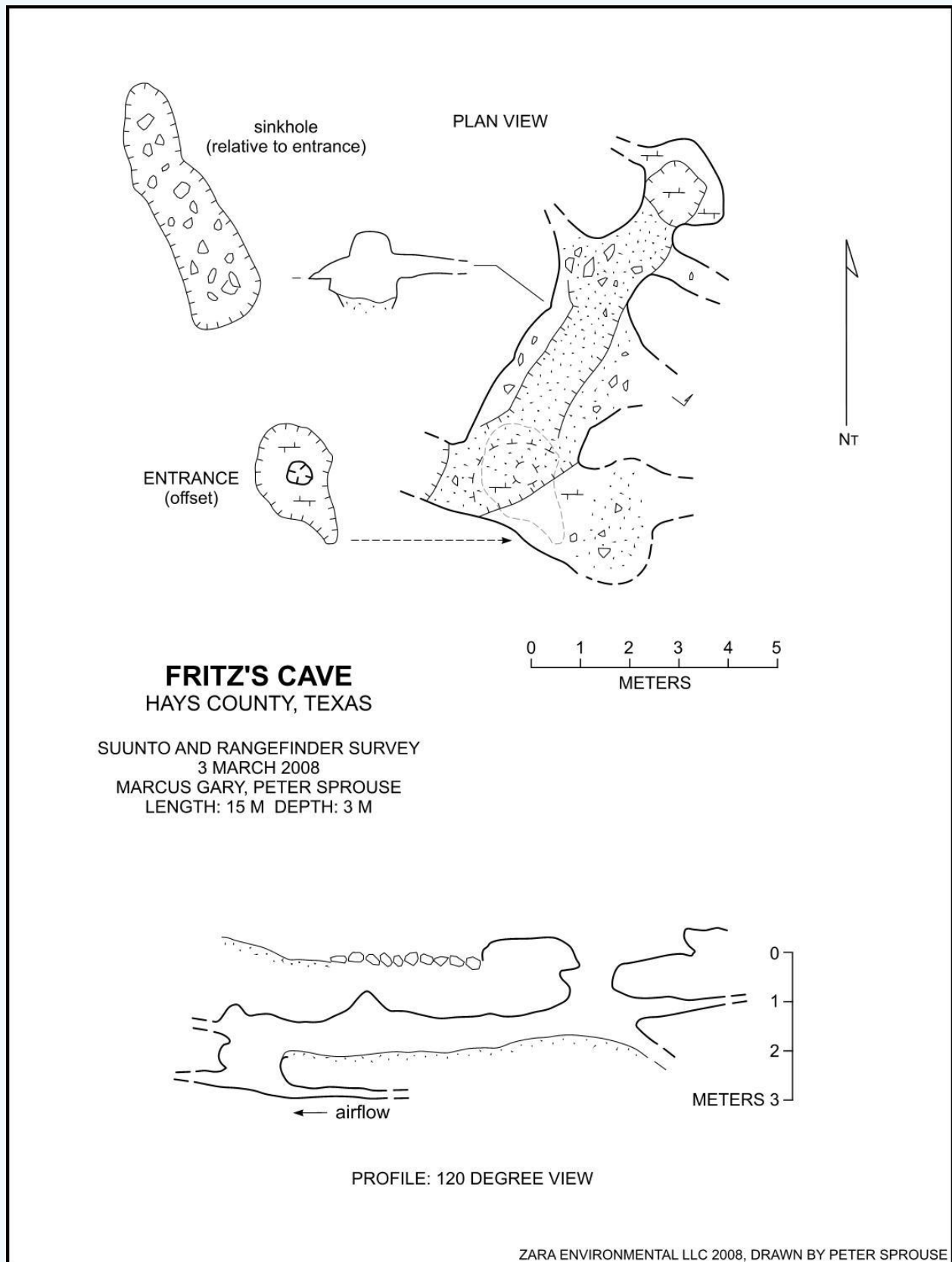
Figure 40. Map of Fritz's Cave
