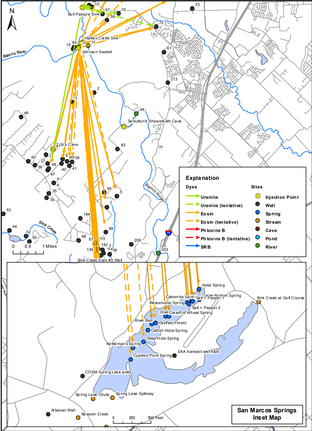
Figure 33. Tracer-Test Results South of the Blanco River from Blanco River Injection Points
