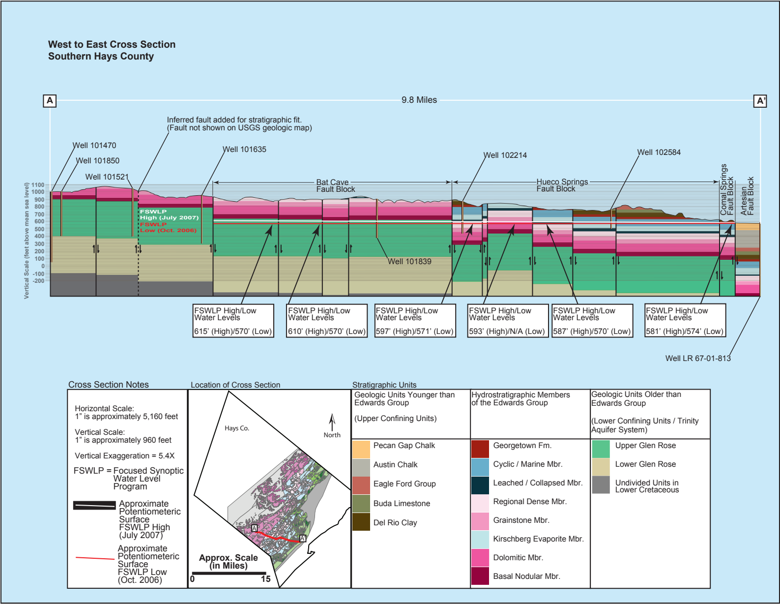
Figure 2. Edwards Aquifer Cross Section near San Marcos Springs
