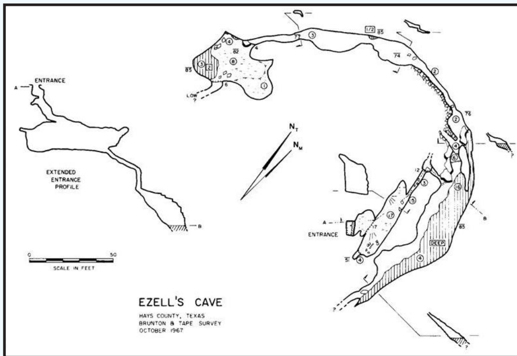
Figure 11. Map of Ezell's Cave
