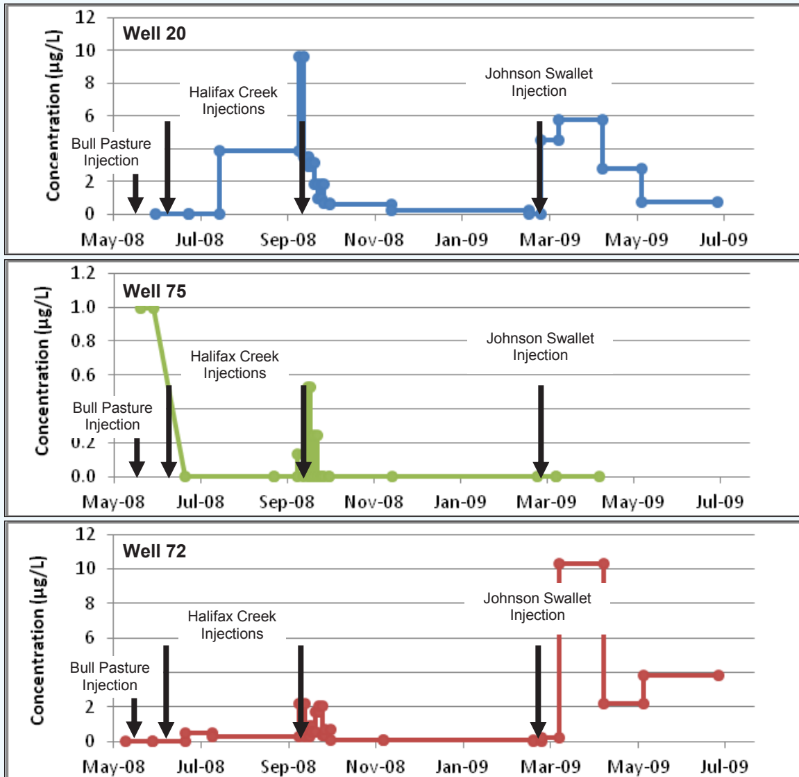
Figure 37. Breakthrough Curves for Wells 20 (5857913), 75 (5857512), and 72 (58579MW) in Charcoal Receptors
