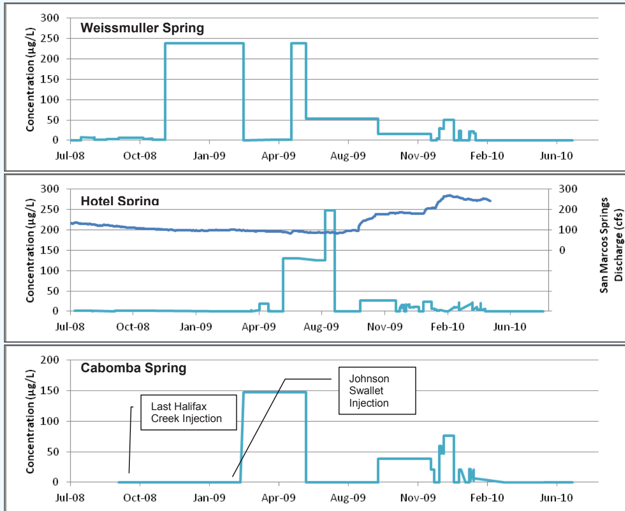
Figure 38. Eosin Concentrations at Weissmuller, Hotel, and Cabomba Springs in Charcoal Receptors
