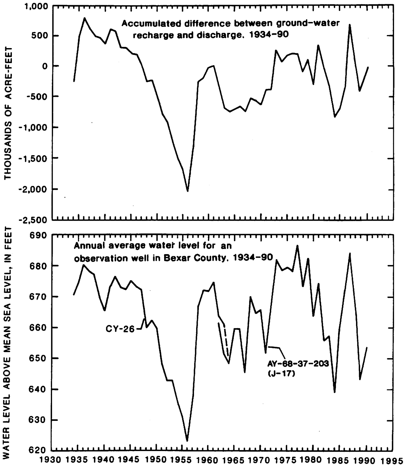
Figure 5.--Accumulated difference between ground-water recharge and discharge, and annual average water level for an observation well in Bexar County, 1934-90.
