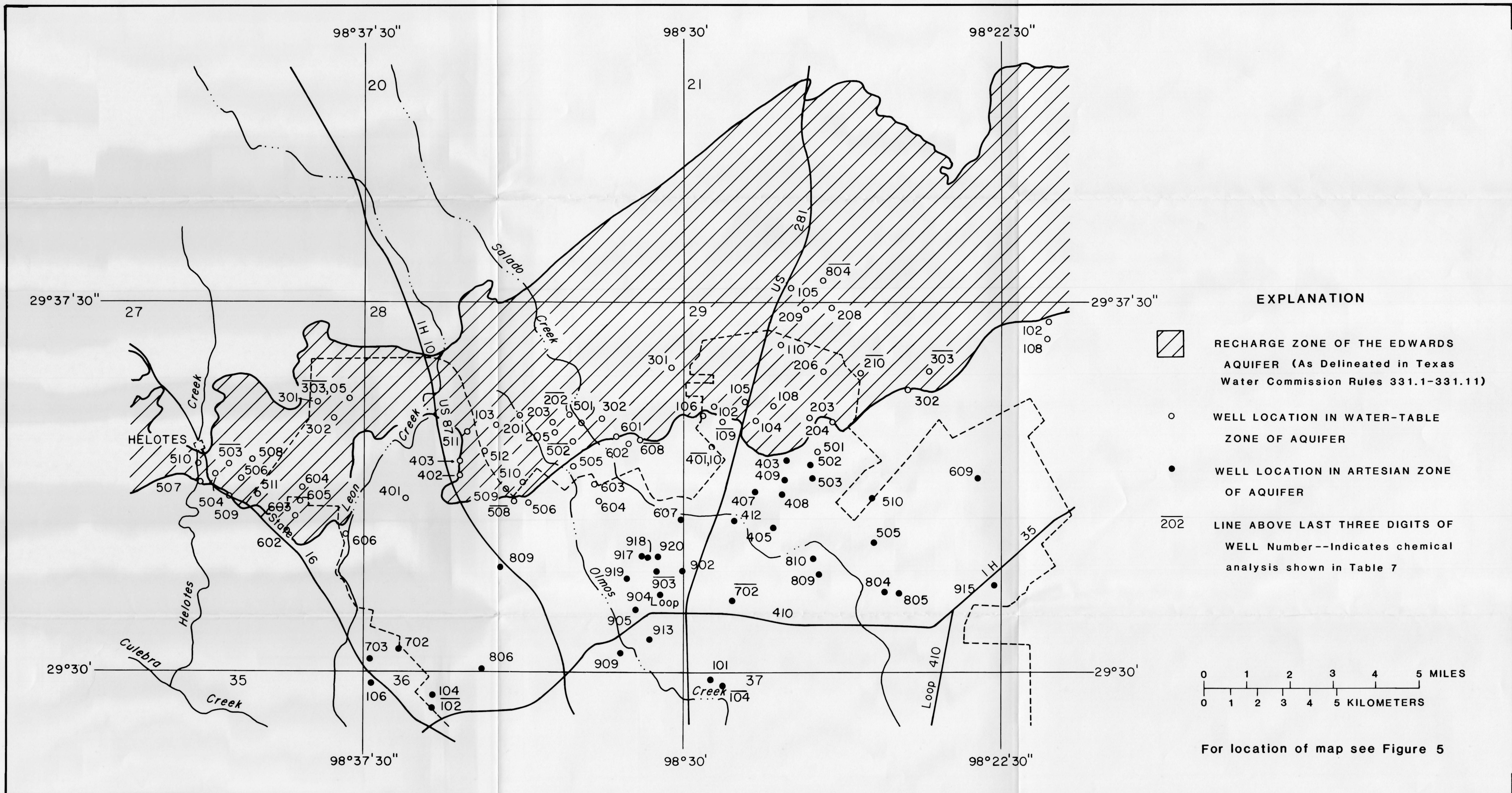
Figure 6.--Location of water-quality data-collection sites for wells and springs in the Edwards aquifer in the San Antonio area that have been sampled since 1968
