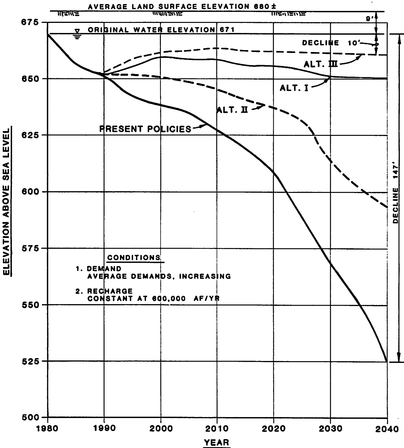
FIGURE 5-5 ALTERNATIVE WELL WATER LEVELS IN SAN ANTONIO AREA
