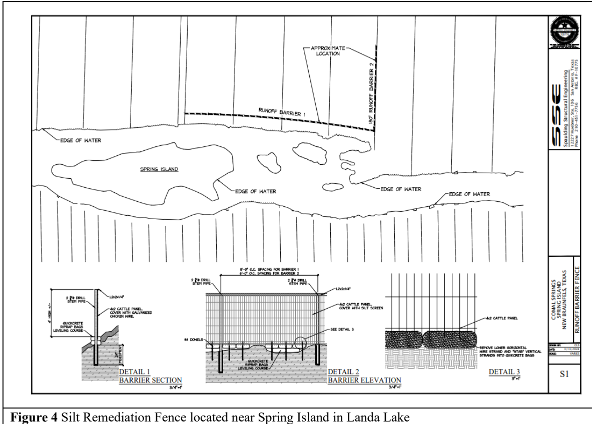
Figure 4 Silt Remediation Fence located near Spring Island in Landa Lake
